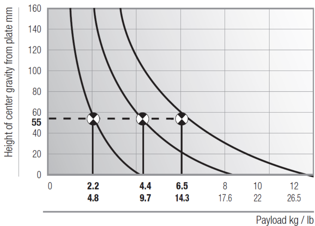
COUNTERBALANCE GRAPH
