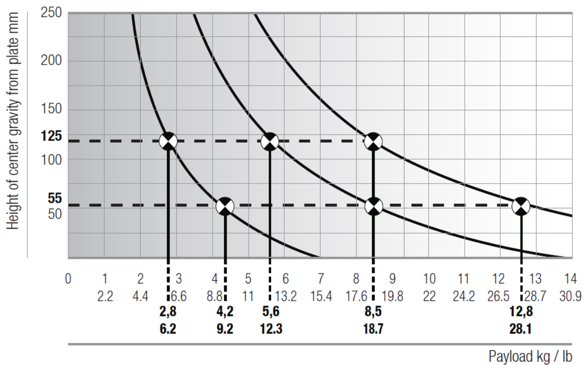
COUNTERBALANCE GRAPH
