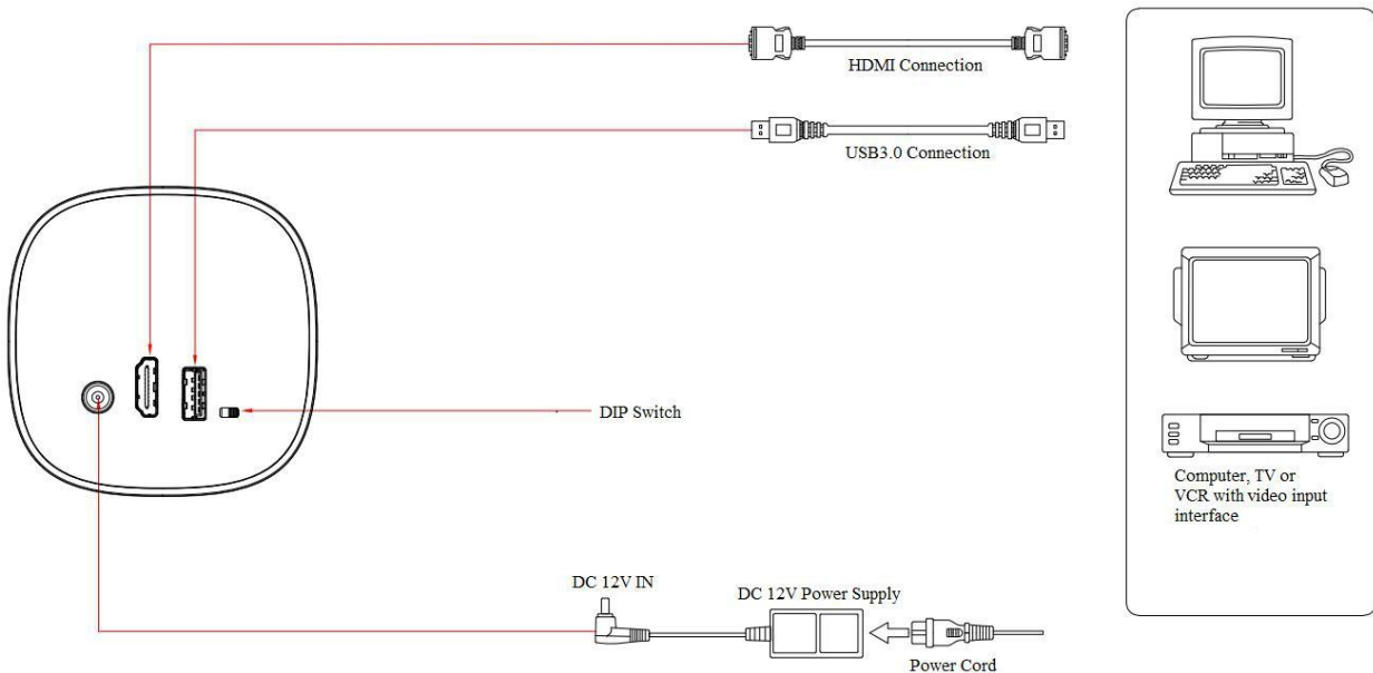
Figure1-3 Wiring Diagram
