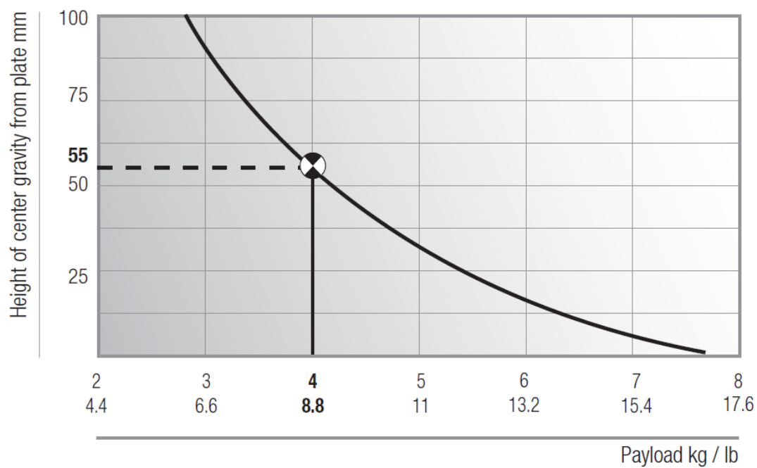
COUNTERBALANCE GRAPH
